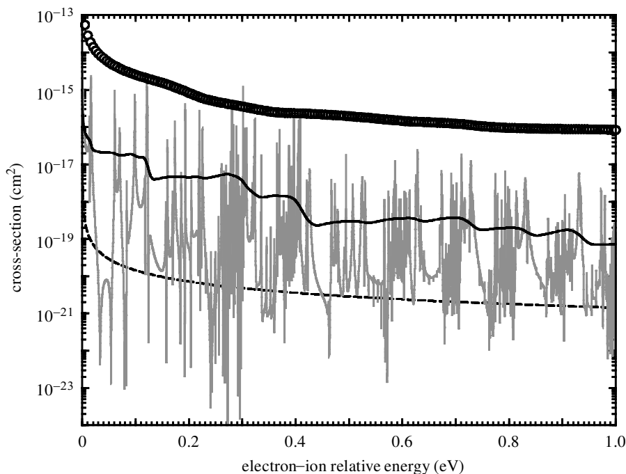
Figure 4. DR of \text{H}_3^+ at low energy, modelled within a combined MQDT–wave packet approach. The dashed black line denotes the computed direct cross-section. The grey line denotes the computed total (direct and indirect) cross-section. Circles denote CRYRING measurements (Larsson et al. 1997). The solid black line denotes the computed total cross-section, convoluted according to the anisotropic Maxwell distribution characterizing the ions in the CRYRING experiment (Larsson et al. 1997). The computations are performed in the C_{2v} symmetry and are restricted to the contribution of the p^2B_2 continuum of the ‘ion-plus-electron’ system.
